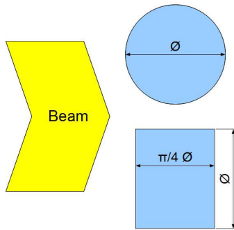
(a) Approximation of a rectangular wire cross section of the proper surface.
