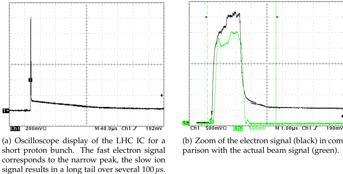
Figure 2.4: The LHC IC signal for a short bunch of protons of 1.7 \mu s [50].
