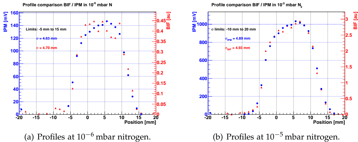
Figure 4.20: Comparison of beam profiles acquired by the IPM (blue) and the GSI BIF monitor (red).
