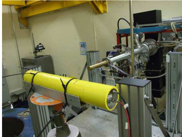
Figure 2.7: Photo of the experimental setup at the SAMES accelerator at CEA Valduc, in yellow the IC in the background the accelerator with the D/T-target.
