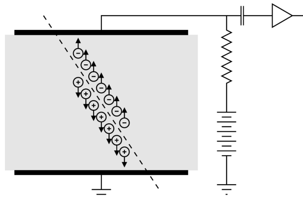
Figure 2.21: An ionizing particle passes through a diamond detector. It generates electron-hole pairs that are extracted by an electric field applied over electrodes on top and on bottom [60].
