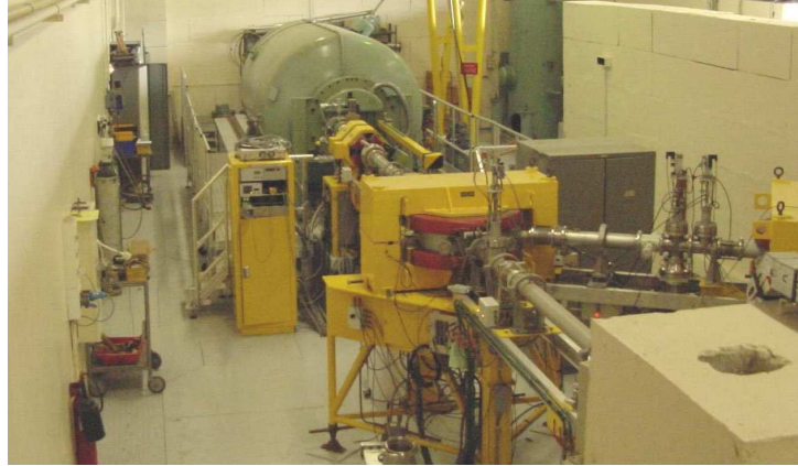
Figure 2.28: Photo of the Van de Graaff accelerator at CEA Bruyères-le-Châtel [72].
