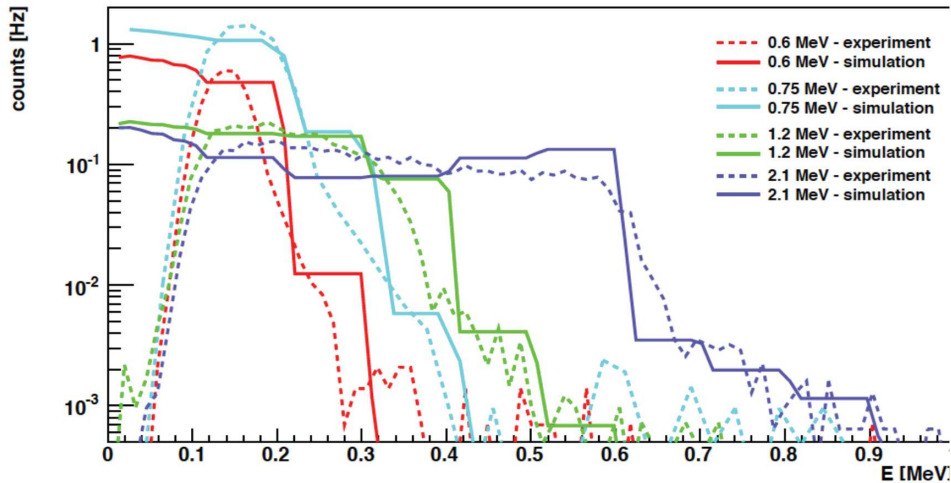
Figure 2.30: Comparison of the energy loss spectra of neutrons of various energies measured at B3 with Simulation.
