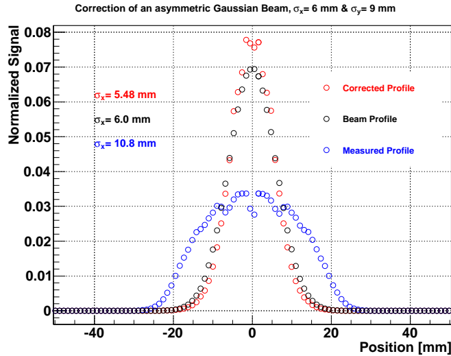
Figure 4.57: SC correction of the x-profile of a Gaussian asymmetric beam of \sigma_x = 6 \text{ mm} & \sigma_y = 9 \text{ mm} .
