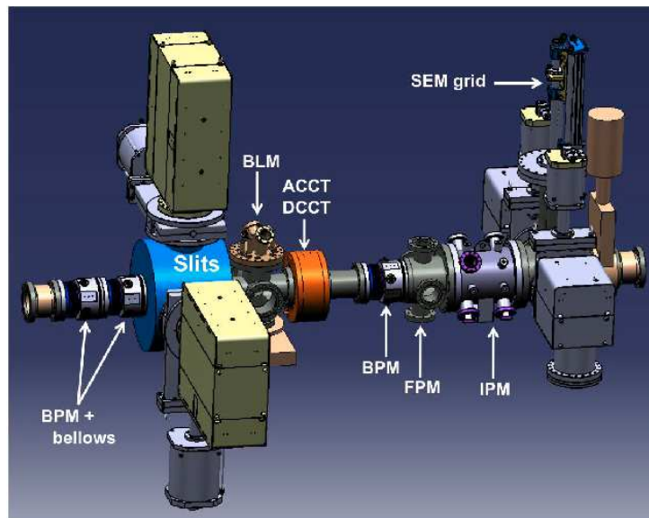
Figure 1.18: Diagnostics foreseen on the D-plate: In charge of CEA Saclay: ACCT and DCCT, SEM grid, and IPM, in charge of CIEMAT Madrid: BPMs, slits, FPM profiler, and in charge of INFN Legnaro: Bunch Length Monitor (BLM) .
